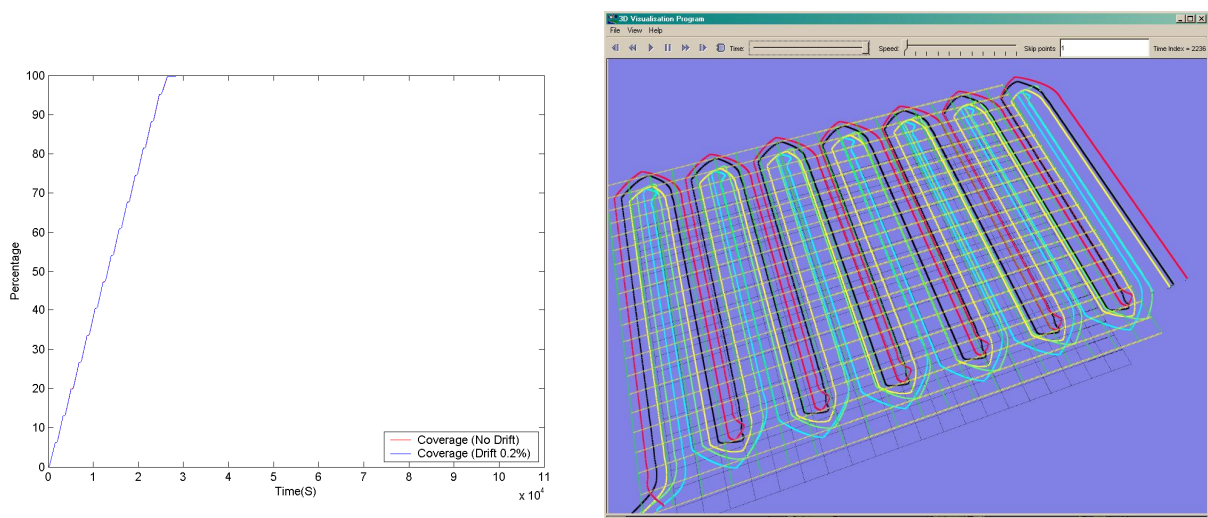
Fig 3. (Left) Coverage over time of a swarm of 5 UUVs, while formation flying with drift set as 0.2% and no drift. (Right). Trajectory of the formation flying case with drift (2%) that was not reset periodically.
