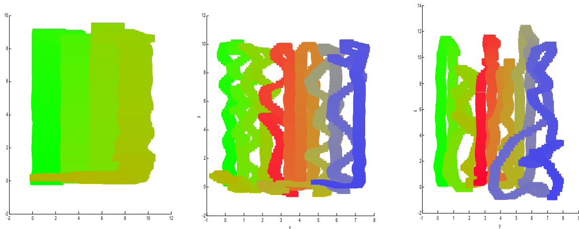
Fig 12. (Left) Coverage of a single aerobot with swath of 2.8m and line spacing of 2.5m. (Middle) Coverage of non cooperative UUVs with swath width of 0.625m. (Right) Coverage of cooperative aerobots with swath width of 0.625m.
