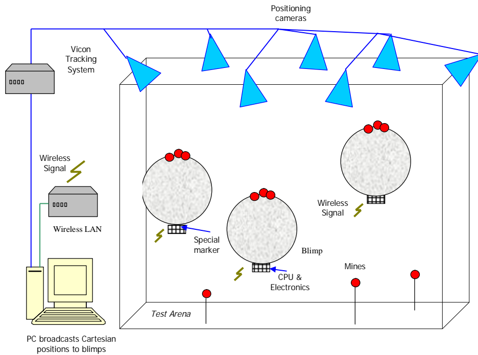
Fig 10. Vicon system and the test environment setup.
