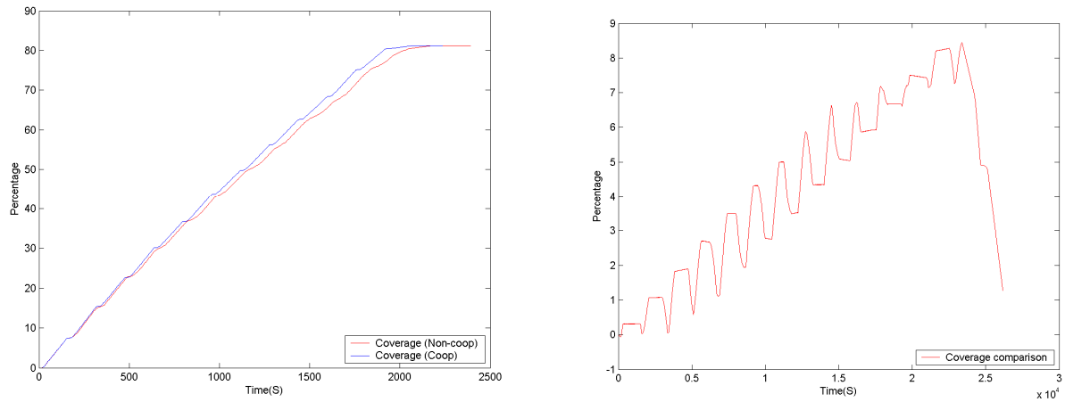
Fig 4. (Left) Coverage comparison between formation flying and non-cooperative behaviours with drift set at 2% (without reset). (Right). The difference in coverage over time.
